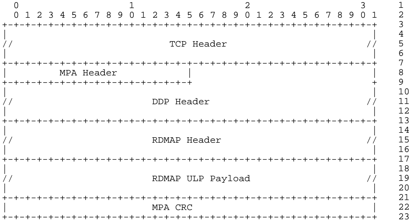
Figure 2 MPA, DDP, and RDMAP Header Alignment
