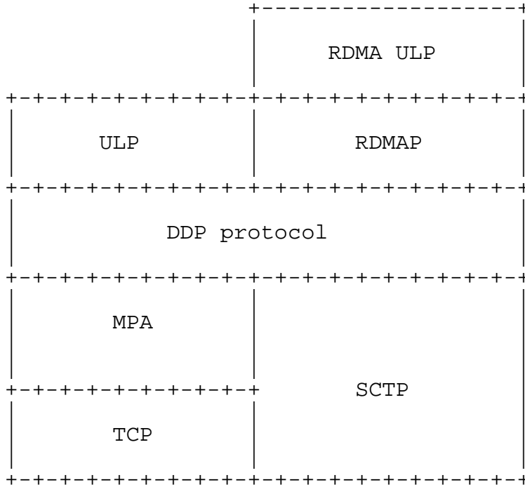
Figure 1 DDP Layering
